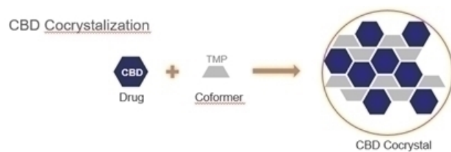
Blockbuster Cocrystals
